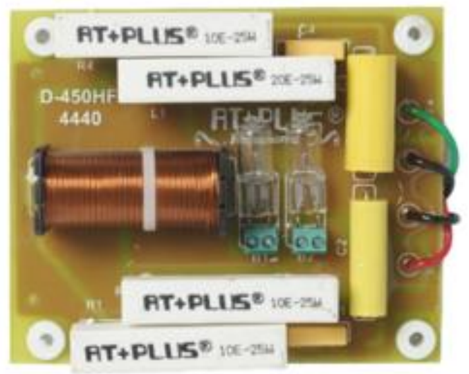
AT – D-450
